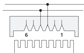
Rear View of Terminal Connection Block
