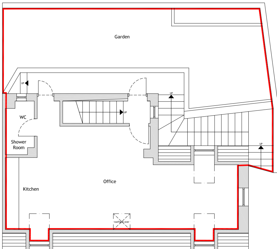
+02 Second Floor Plan
